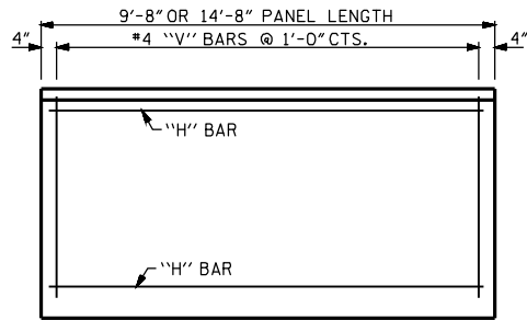
FRONT ELEVATION OF UPPER PRECAST PANELS
