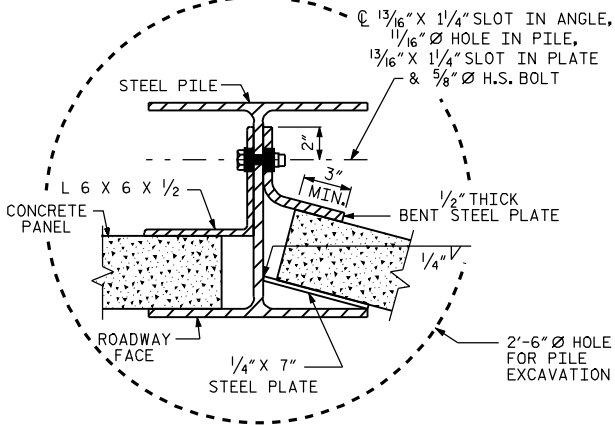
TYPICAL WALL TURN DETAIL
