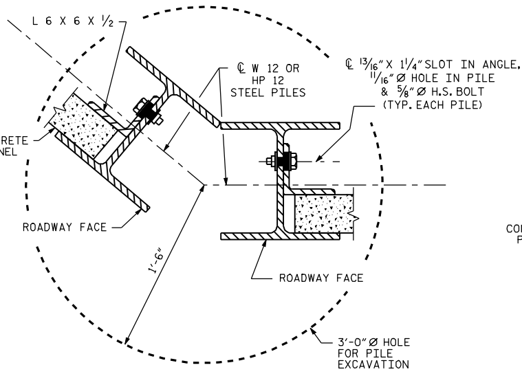
TYPICAL WALL TURN DETAIL
