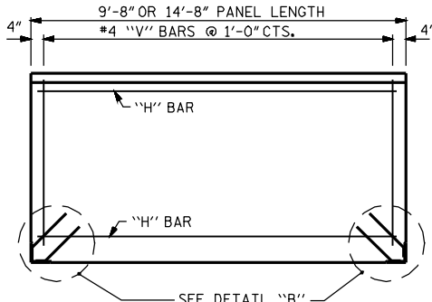
FRONT ELEVATION OF BOTTOM PRECAST PANEL
